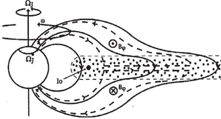
Figure 1.11: Meridian cross through the Jovian magnetosphere showing the field-aligned current system (dotted lines). The dotted region indicates the plasma. \Omega_J is the angular velocity of the planet, \omega is the angular velocity of a shell of field lines and \Omega_J^* is the angular velocity of the Pedersen layer (Cowley and Bunce 2001).
