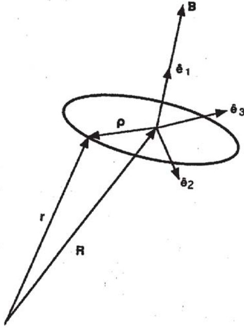
Figure A.1: Coordinate system for particle gyration in an inhomogeneous magnetic field.
