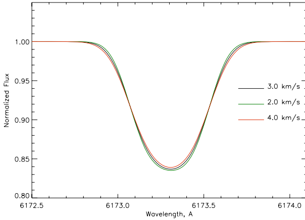
Figure 3.14: Spectral line profiles of Fe I (6173.33 Å) line calculated with v \sin i = 27.5 km/s and 3 different values of the macro-turbulence. The red line represents the line profile calculated with \zeta = 4.0 km/s, the green line with \zeta = 2.0 km/s and the black line with \zeta = 3.0 km/s
