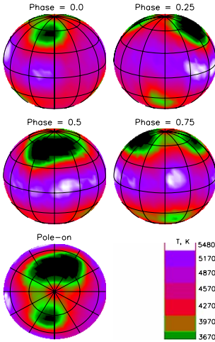
Figure 3.34: Reconstructed surface map of \sigma Gem for v \sin i = 25.0 km/s is shown in four orbital phases with a coordinate grid of 30^\circ in both latitude and longitude. Plotted is the effective temperature distribution given by the colour scale, which is given by the bottom right panel.
