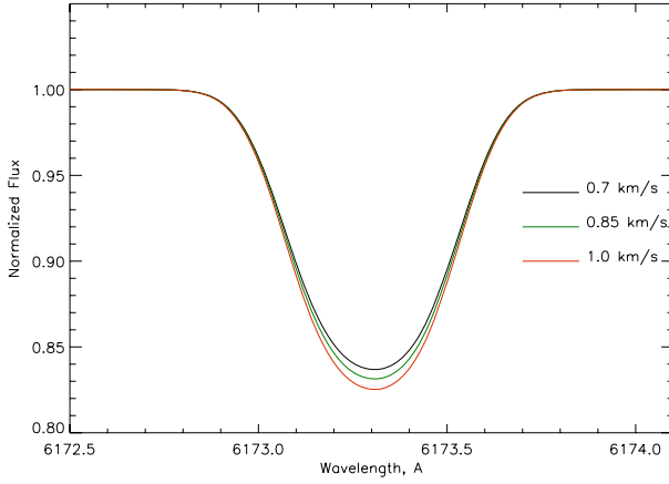
Figure 3.13: Spectral line profiles of Fe I (6173.33 Å) line calculated with v \sin i = 27.5 km/s calculated with 3 different values of the microturbulence. The red line represents the line profile calculated with \xi = 1.0 km/s, the green line with \xi = 0.85 km/s and the black line with \xi = 0.7 km/s
