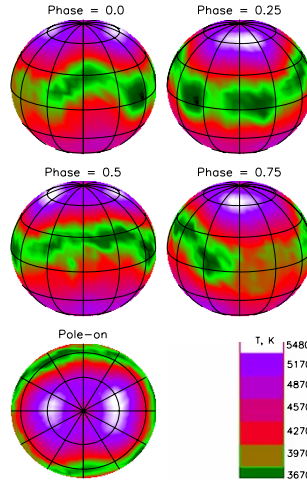
Figure 3.35: Reconstructed surface map of \sigma Gem for v \sin i = 30.0 km/s is shown in four orbital phases with a coordinate grid of 30^\circ in both latitude and longitude. Plotted is the effective temperature distribution given by the colour scale, which is given by the bottom right panel.
