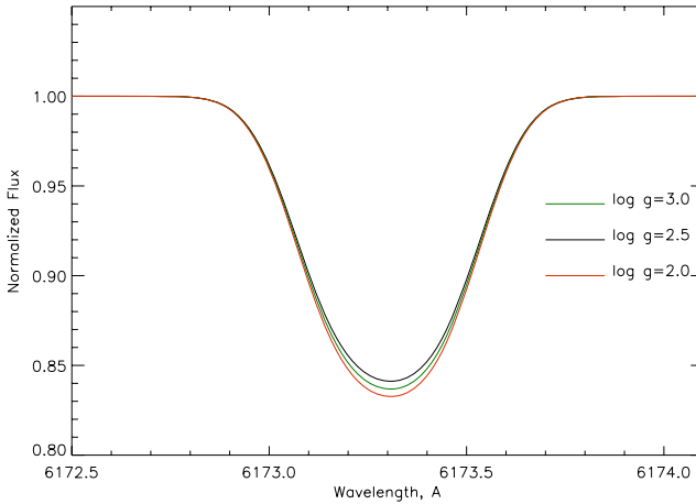
Figure 3.6: Spectral line profiles of Fe I (6173.33Å) line calculated with v \sin i = 27.5 km/s calculated with 3 different \log g . The red line represents the line profile calculated with \log g = 2.0 , the black line — with \log g = 2.5 and the green line — with \log g = 3.0
