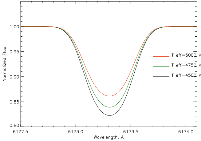
Figure 3.19: Spectral line profiles calculated with 3 different values of the effective temperature. The red line represented the line profile calculated with T_{\text{eff}} = 5000 K, the green line with T_{\text{eff}} = 4750 K and the black line with T_{\text{eff}} = 4500 K
