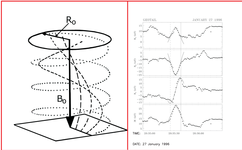
Figure 1.12: Schematic depiction of a helical flux rope (left panel) and in situ observations of a flux rope in the magnetotail (right panel) [Slavin et al. , 2001].
