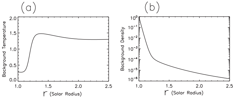
Figure 2.5: Background temperature (a) and density (b) as a function of radial coordinate in units of the solar radius. [Ruan, et al. , 2008]
