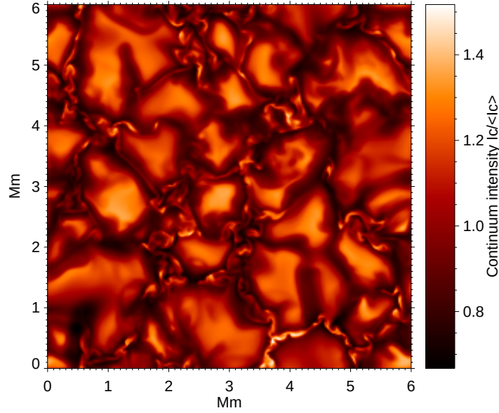
Figure 4.1: Normalized continuum intensity map near 6302 Å emerging from the simulation box at disc center.
