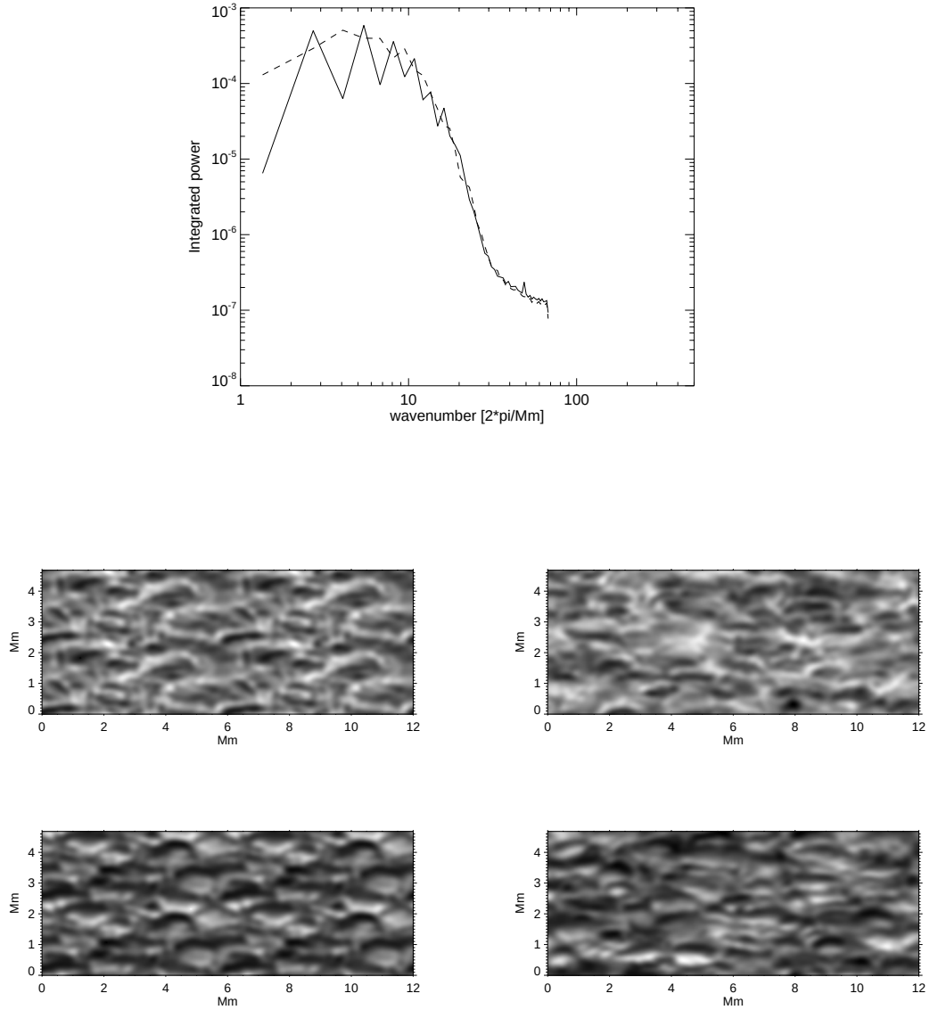
Figure 4.13: Upper panel: integrated power spectra for the two middle images (full line: observations, dashed line: simulations). Middle left panel: simulated Stokes- I maps at -50 \text{ m\AA} from line center Fe I 6302.5 \text{\AA} . Middle right panel: observed Stokes- I maps at -50 \text{ m\AA} from line center Fe I 6302.5 \text{\AA} . Lower left panel: simulated Stokes- I maps at +50 \text{ m\AA} from line center Fe I 6302.5 \text{\AA} . Lower right panel: observed Stokes- I maps at +50 \text{ m\AA} from line center Fe I 6302.5 \text{\AA} .
