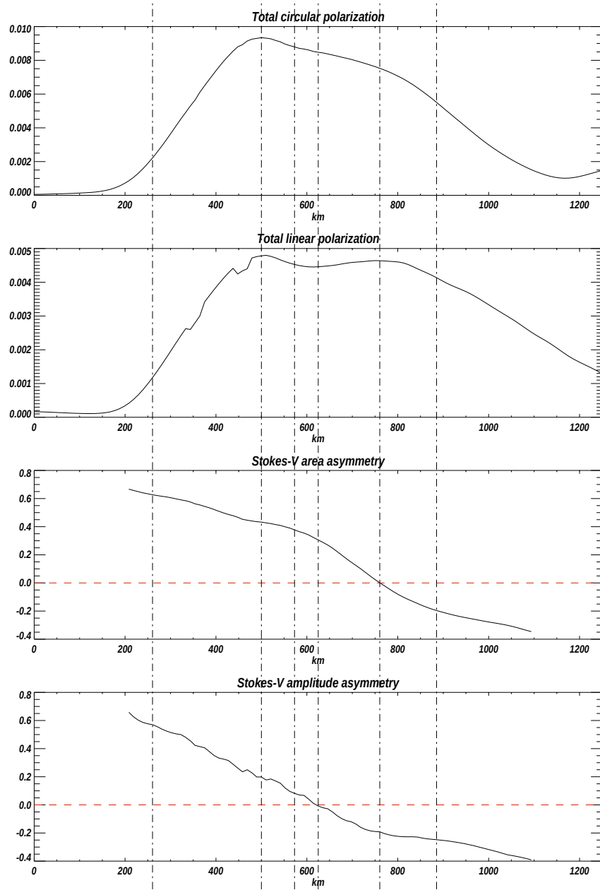
Figure 4.8: From top to bottom : Total circular polarization, total linear polarization, Stokes-V area asymmetry, and Stokes-V amplitude asymmetry, all plotted along the atmospheric slice in Figure 4.7. The vertical dash-dotted lines indicate the same locations shown by vertical lines in the previous figure.
