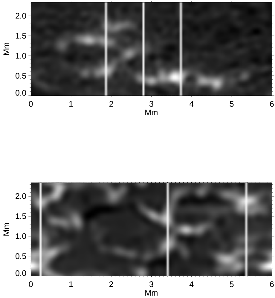
Figure 4.14: Upper panel: observed Stokes-V at -50 \text{ m}\text{\AA} from line center FeI 6302.5 \text{\AA} . Lower panel: Stokes-V from simulations degraded to the resolution of observations. White slits indicate the positions where we plot the Stokes-V signal in Figure 4.15.
