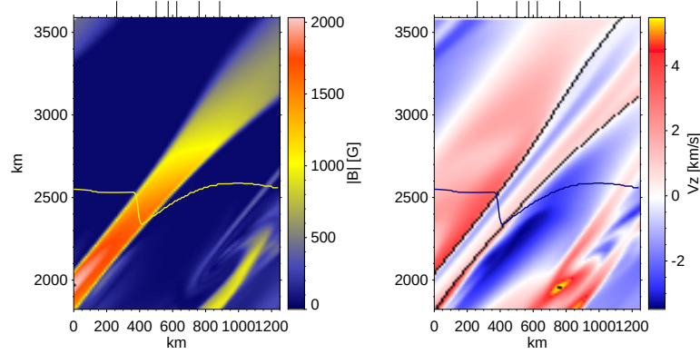
Figure 4.7: 2D inclined view at \mu = 0.39 of the magnetic flux element shown in Figure 4.3. The magnetic field strength is shown in the left panel. The line-of-sight velocity is represented in the right panel, where red and blue shifts are represented in red and blue colours respectively. The optical depth \tau = 1 is shown by the yellow and blue lines. The boundaries of the flux element are highlighted in black in the velocity panel. The small vertical lines on the top of the two images indicate the locations of rays analysed in more detail in Figure 4.11
