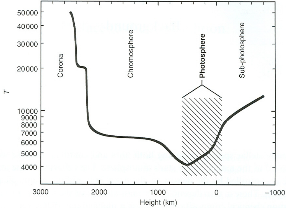
Figure 1.1: The height distribution of temperature in the outer layers of the sun. The height is given in kilometers measured from a zero point where the average optical depth < \tau_{5000} > = 1 . The photosphere is indicated by the shaded region. Adapted from Gray 2005, based on the work of Vernazza et al. (1973).
