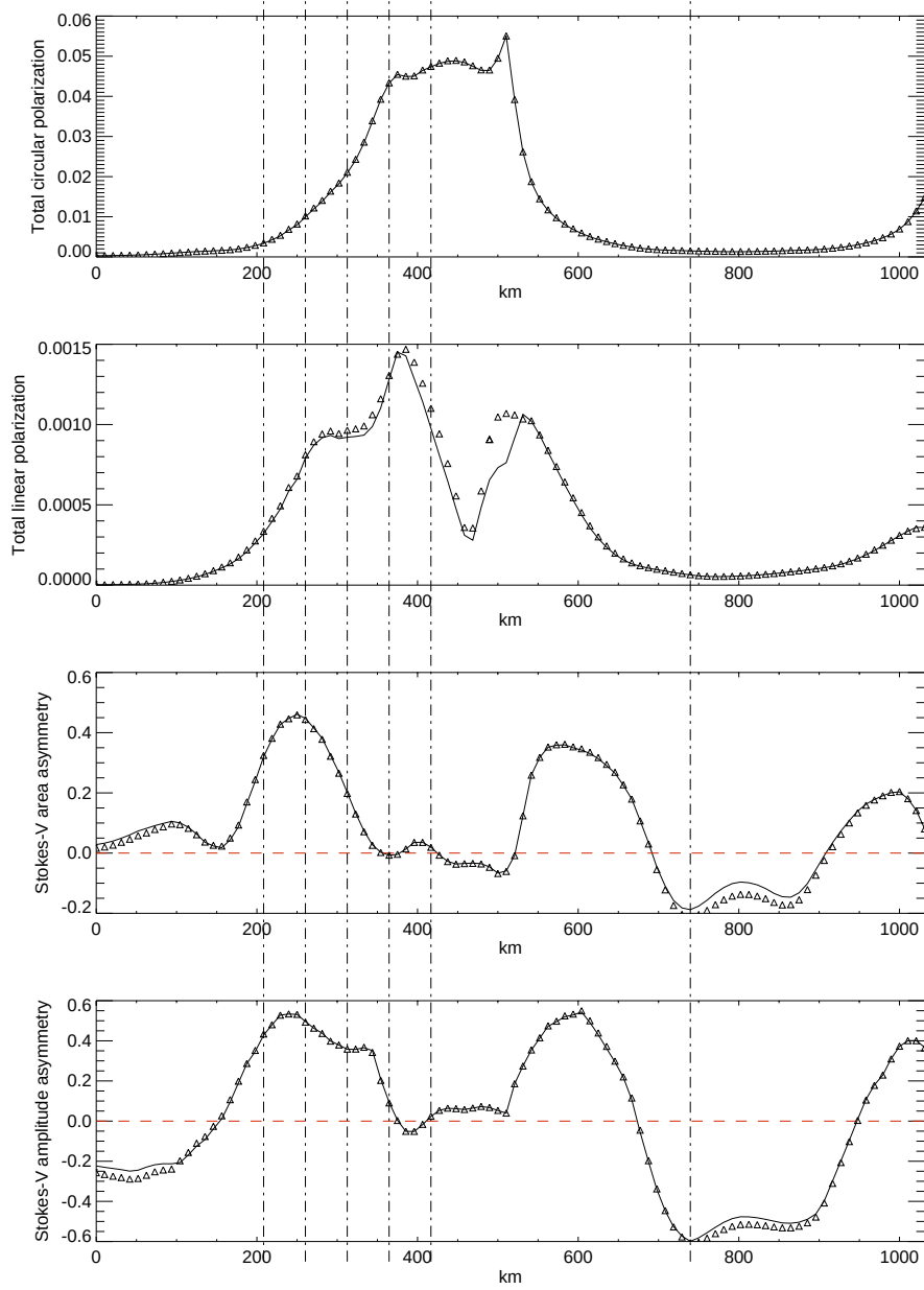
Figure 4.4: From top to bottom (in full lines): Total circular polarization, total linear polarization, Stokes-V area asymmetry, and Stokes-V amplitude asymmetry, all plotted along the black line on Figure 4.2. The curves indicated with triangles represent the same plotted quantities but calculated without magneto-optical effects. The vertical dash-dotted lines indicate the same locations shown by vertical lines in the previous figure.
