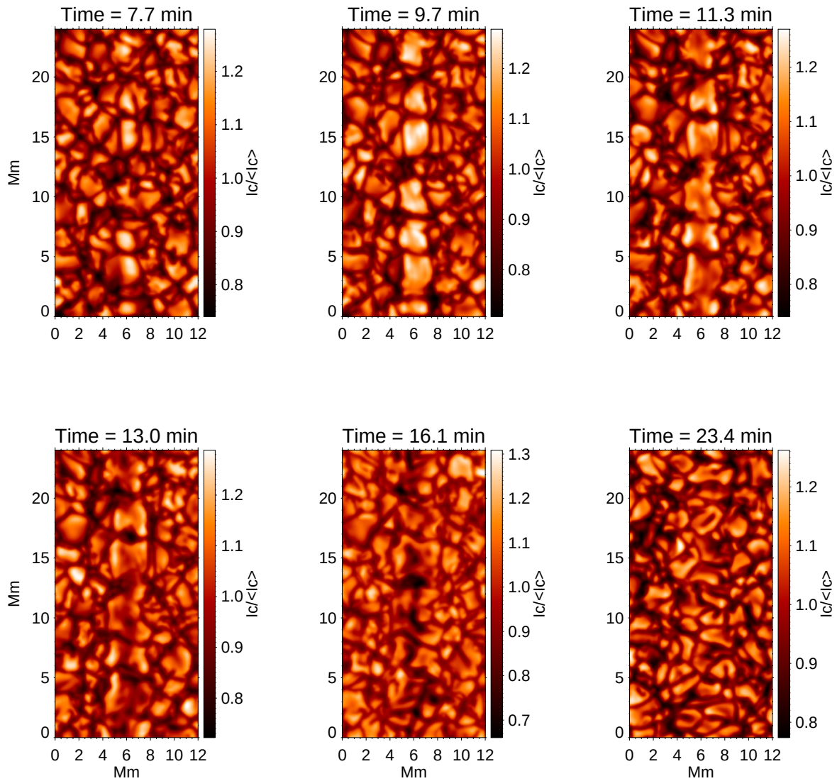
Figure 5.1: Time sequence of normalized continuum intensity maps near 5000Å covering the flux tube's emergence at the solar surface. The time is counted starting from the introduction of the flux tube at -1.35 Mm below the visible solar surface. The images are degraded to Hinode's SP resolution
