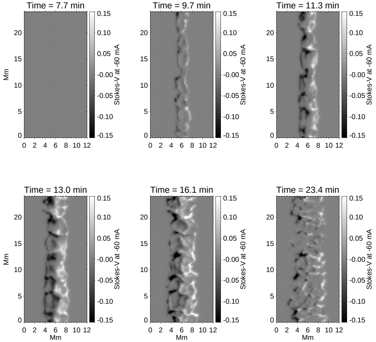
Figure 5.2: Time sequence of maps showing the Stokes-V signal at -60 \text{ mÅ} from the line center of Fe I 6302.5 \text{ Å} . The signal is clipped to \pm 0.15 I_c , with I_c being the local continuum intensity. The images are degraded to spatial and spectral conditions similar to Hinode's SP near 6302.5 \text{ Å} . Individual snapshots refer to the same times as those of Figure 5.1.
