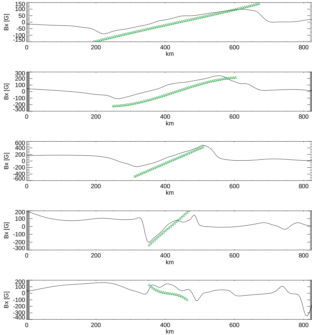
Figure 3.11: Horizontal component of the magnetic field across the flux sheet plotted along the 5 horizontal cuts in Figure 3.5. The green triangles represents B_x in the case of a 2 nd -order thin flux sheet model.
