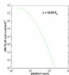
Exosphere Model
