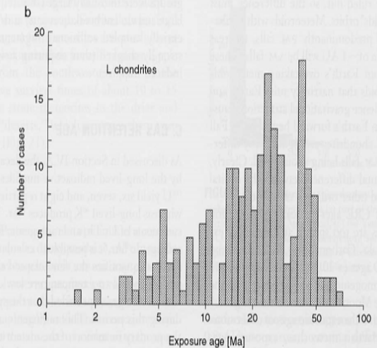
FIGURE 22 Cosmic ray exposure ages for ordinary (a) H, (b) L, and (c) LL chondrites. Peaks in the histograms indicate major collisional events on parent bodies that generated substantial proportions of meter-sized fragments (see Section V, B).
