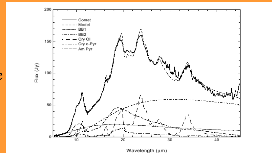
Fig. 2. ISO SWS spectrum of Comet Hale-Bopp at r = 2.8 AU, degraded to \lambda = 500 , compared with a five-component dust model: 280 K blackbody (BB1); 165 K blackbody (BB2); forsterite (Cry Ol 22%); orthopyroxene (Cry o-Pyr 8%); and amorphous pyroxene (Am Pyr 70%). From Crovisier et al. (2000).
