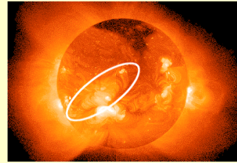
Loop arcade
