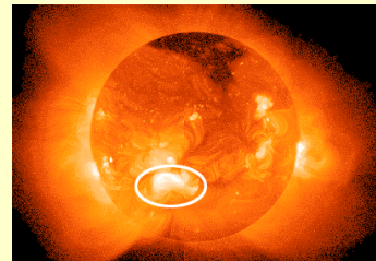
Active zone
