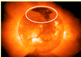
Coronal hole
