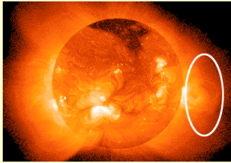
Isolated loop
