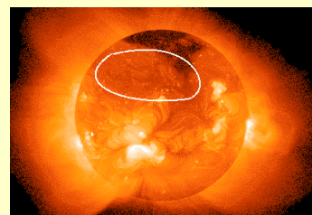
Quiet zone
