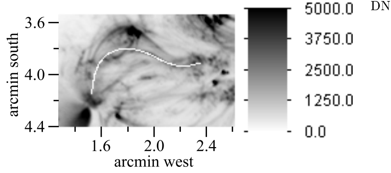
Figure 6.2: Region of interest with the loop analysed in this chapter, as seen in channel AIA 171. The field line used for the analysis is overplotted.
