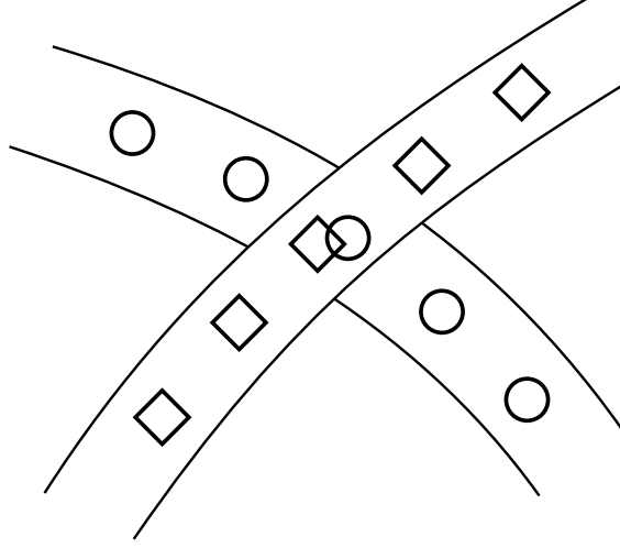
Figure 8.2: Two crossing loops with sample points placed on them. As the iterative updates are smoothed along the loops, the two sample points in the crossing can develop differently (from Barra, re-submitted to Solar Physics).
