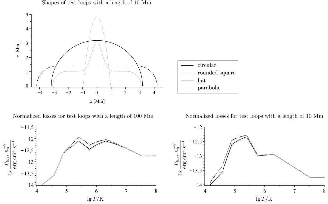
Figure 7.14: The normalized radiative losses P_{loss}(T)/n_0^2 for four loops with constant temperatures, but different shapes (bottom panels). Displayed are the cases of different loop lengths. Top panel: The shape of the loops. The different line styles and colours refer to the same shapes in each panel.
