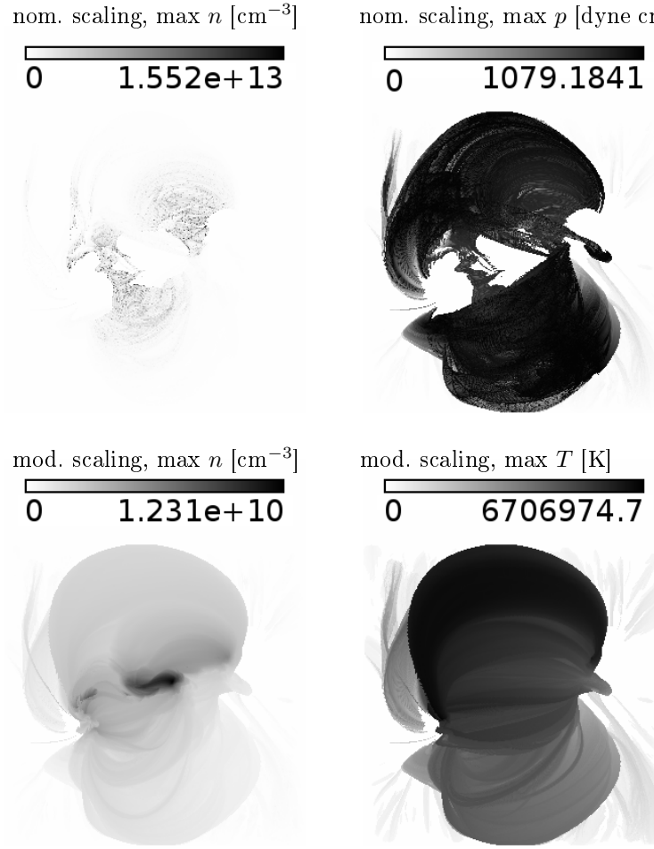
Figure 7.12: Physical conditions from the model Serio et al. 1982 + Golub et al., 1982, with NLFFF. Top: the nominal scaling of Golub et al., 1982. Bottom: the scaling where the pressure is divided by 1000.
