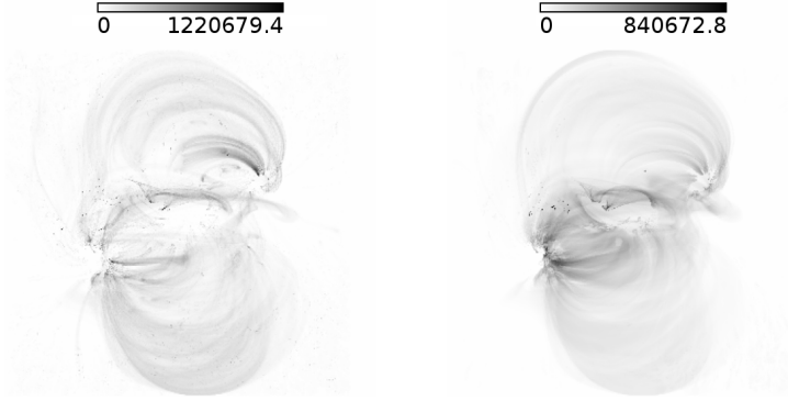
Figure 7.5: The RTV78 + Golub et al., 1982 model and a NLFFF, but without the emission from loops that are rooted in regions of at least 500 Gs with both foot points. Left: Lower boundary set to z = 0 , right: lower boundary set to z = 5 .
