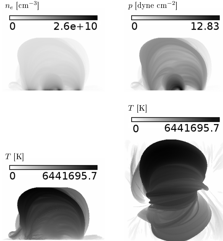
Figure 7.7: Physical conditions in the model atmosphere resulting from RTV78 + modified Golub et al., 1982, with the NLFFF and the lower boundary set to z = 5 . Displayed are the maximum of the density, the pressure the temperature, respectively. The lower right picture has the same LOS as the observations. All other pictures feature a horizontal view from south to north.
