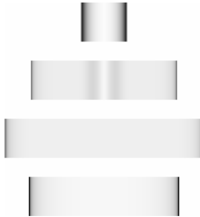
Figure 7.13: Modelled intensities (in a.u.) of four hypothetical loops of the same length. The loops have the same constant temperature and a constant density everywhere. They only vary in shape (fig. 7.14), yielding different appearances. These images are negative images, i.e. darker regions here are actually brighter.
