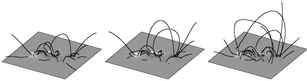
Figure 2.5: Twenty field lines for different magnetic field models for AR 11158, Feb. 14th, 2011, extrapolated from the same foot points. From left to right: potential field, linear force-free field with \alpha = 2 , non-linear force-free field. The differences are striking (own work, field extrapolations courtesy T. Wiegelmann).
