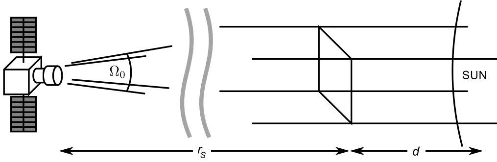
Figure 4.3: Schematics of a pixel's field of view. The pixel observes a solid angle of \Omega_0 . Since the sun is far away, and the observed part of its atmosphere is thin compared to the distance ( r_s \gg d ), the line of sights might be considered parallel on the sun (own work).
