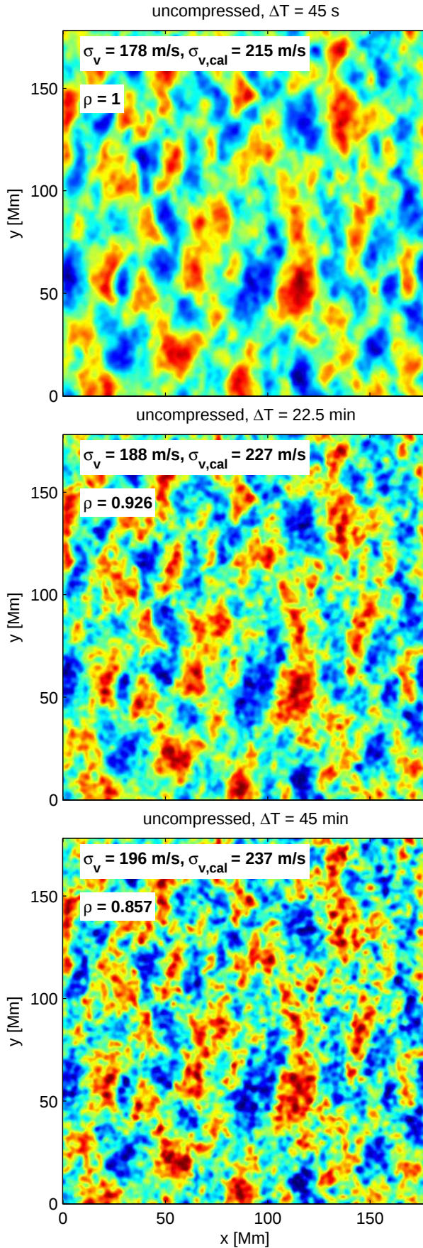
Figure 4.2: Flows in the x-direction at disk center, as determined by local correlation tracking of granulation (averaged over 24 h). Here and in Figures 4.3 and 4.4, we compare a flow map for uncompressed data with flow maps for different compression methods. In the vertical direction, we vary the time lag \Delta T between consecutive velocity maps used for averaging over 24 h ( top row : \Delta T = 45 s, middle row : \Delta T = 22.5 min, bottom row : \Delta T = 45 min). The flow maps shown in this figure are derived from uncompressed intensity images. Figure 4.3 is for quantized data ( n = 2 ) and Figure 4.4 is for JPEG compression (quality = 10). All flow maps clearly show supergranulation. We use the same scaling of the colormap for all images, corresponding to the amplitudes of the velocities before applying the calibration factor. The numbers in the images give the standard-deviation of the velocities before ( \sigma_v ) and after ( \sigma_{v,cal} ) applying the calibration factor to the data and the correlation with the LCT maps computed from uncompressed data ( \rho ). The flow maps computed from compressed data have a higher noise level than those for uncompressed data. Quantization and JPEG lead to noise in the cross-covariances used by the LCT code and, thus, results in noise that varies on a pixel-by-pixel scale. JPEG causes a higher noise level than quantization. A large time lag between consecutive velocity maps causes granulation noise to remain visible in the image.
