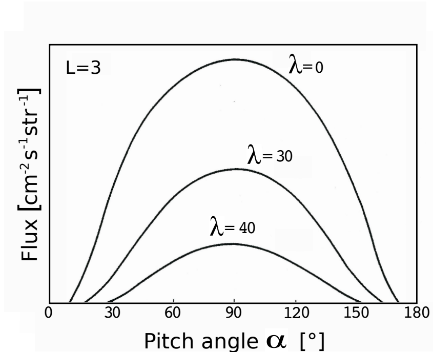
Figure 2.6: Typical pitch angle distributions at L = 3 R_s at three latitudes. With increasing latitude also the loss cone angle increases and the flux at 90^\circ pitch angle decreases (Walt 2005). Here the pitch angle means the local pitch angle.
