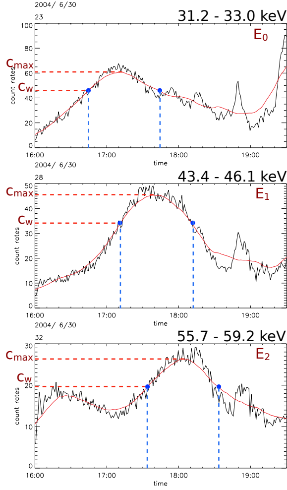
Figure 4.3: Count rates \left[\text{counts sec}^{-1}\right] as a function of time for different PHA energy channels. The injection event (b) of Fig. 4.1 is shown. The red curve represents smoothed data.
