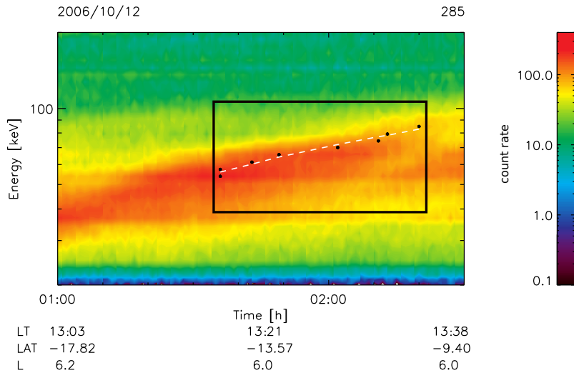
Figure 5.6: Energy time spectrogram of injection event on day 2006/285. The black dots represent the count rate maxima of the different PHA channels, the dashed white line is the fit to the data to obtain E(t) with equidistant time steps.
