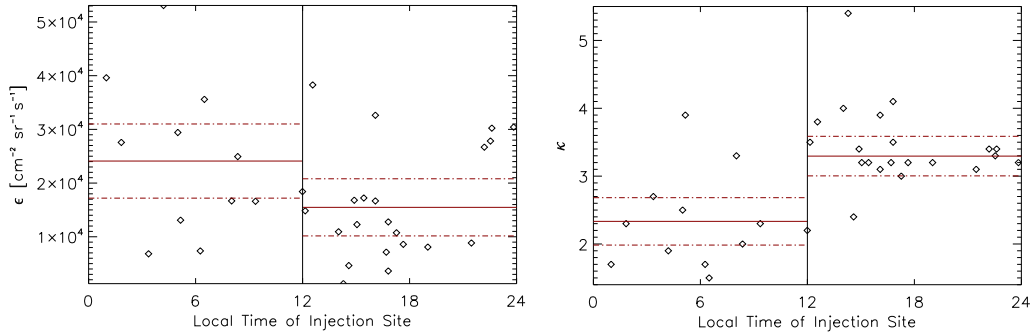
Figure 5.8: \epsilon (left hand side) and \kappa (right hand side) as a function of local time of injection site. The red solid line represents the average value for the two LT sectors, the dotted-dashed line is the standart deviation. For \epsilon the distributions shows higher values in the morning sector (around 6:00 LT) than in the evening sector (around 18:00 LT). For \kappa we find lower values in the morning than in the evening sector.
