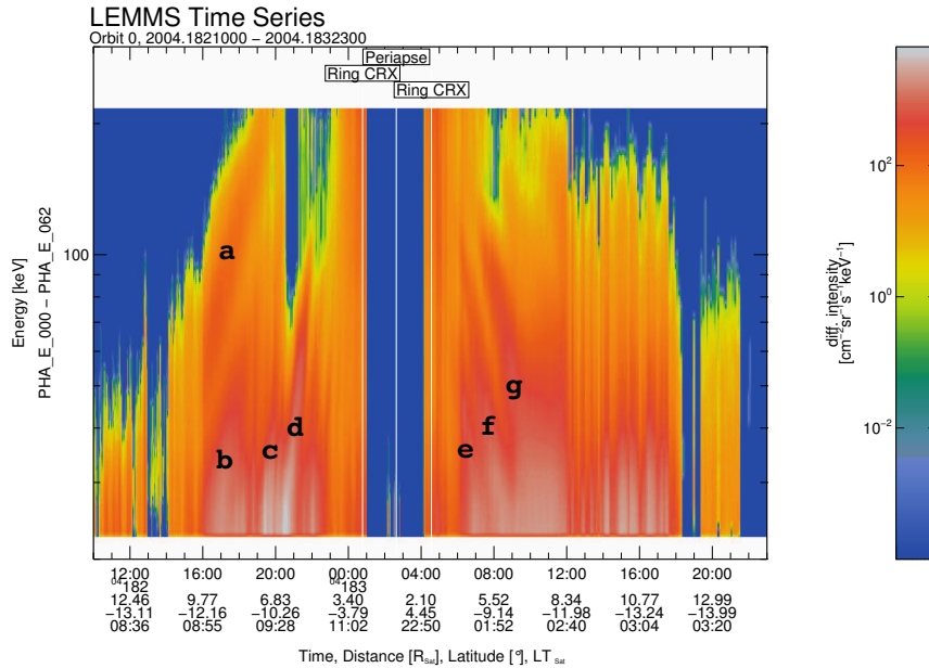
Figure 4.1: Energy-time-spectrogram of Saturn Orbit Insertion (SOI) electron data. Clear signatures of injections are visible around closest approach. ‘Normal’ injections are marked with (a), (b), (c), and (d), the ‘inverted’ events are marked with (e), (f), and (g).
