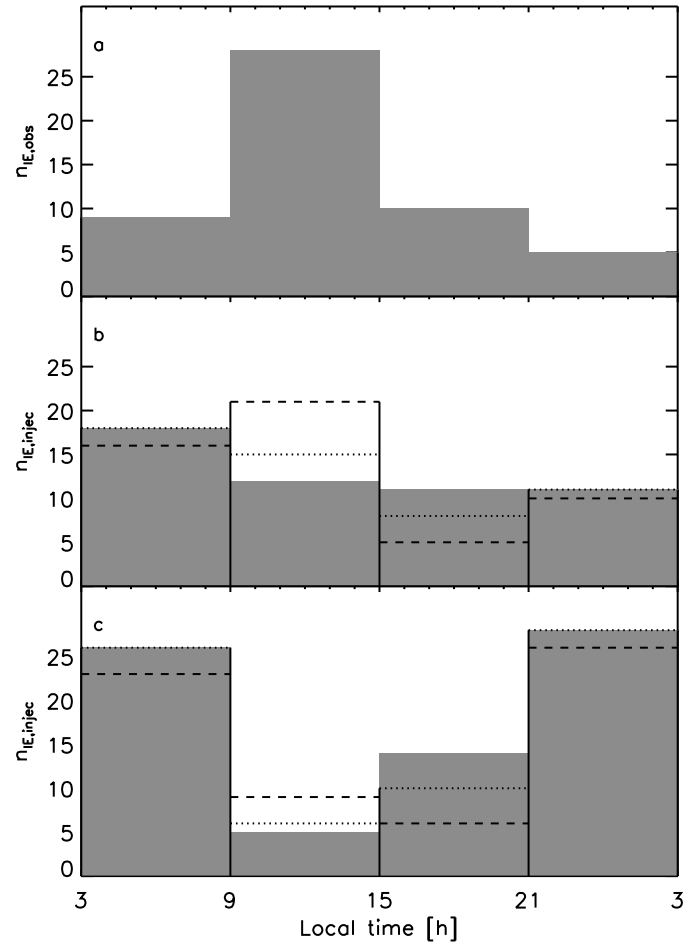
Figure 4.7: Statistical distribution of the number of injection events as a function of the Saturnian local time: (a): distribution of the locations of the measured injections, (b) filled grey: distribution of the origin of the injection site for the calculated angular velocity profile, dashed line: distribution for angular profile (u) in Fig. 4.5, dotted line: distribution for angular profile (l) in Fig. 4.5, (c) weighted distribution of the origin of the injection site for the calculated angular velocity profile, dashed line: distribution for angular profile (u) in Fig. 4.5, dotted line: distribution for angular profile (l) in Fig. 4.5.
