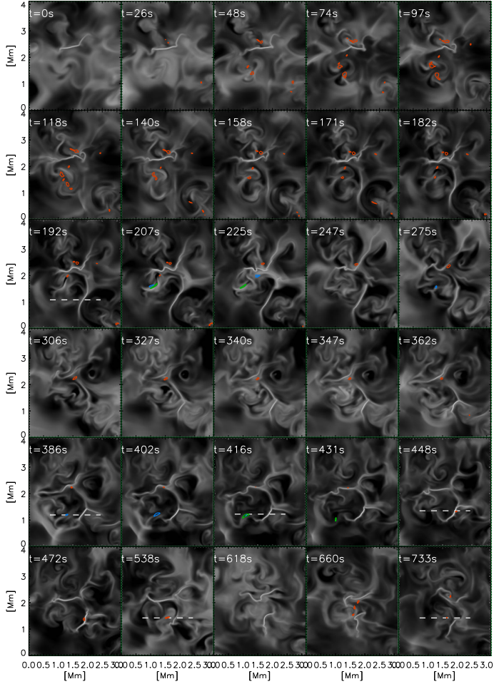
Figure 6.3: Time series of flux-cancellation events. Temperature at \sim 600 km above \langle\tau_{500}\rangle=1 is plotted. Red and blue contours mark dowflow of 5 km/s at \sim 80 km and upflow of 4 km/s at \sim 400 km above solar surface ( \langle\tau_{500}\rangle=1 ), respectively. Green contours outline regions where upflow exceeds 9 km/s at \sim 600 km above the solar surface. White dashed lines show the position of the cuts plotted in Fig. 6.5. The grey scale goes from 3500 K to 8000 K.
