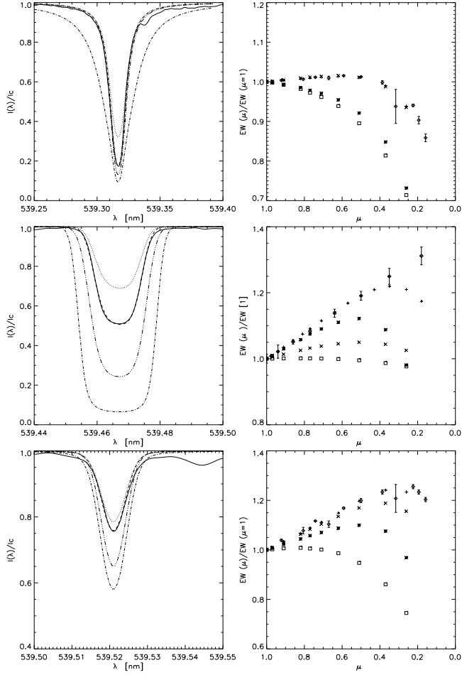
Figure A.2: Left-hand side: Profiles of Fe I 539.32 nm, Mn I 539.47 nm and Fe I 539.52 nm lines at the disk center, from top to bottom respectively. The profiles are computed in the following model atmospheres: quiet Sun (dashed), faculae (dotted), penumbrae (double-dot-dashed) and umbrae (dashed-dotted). FTS atlas profiles are overlotted (solid curves). Right-hand side: Center-to-limb variation of EW of the lines. Symbols distinguish between EW resulting from different model atmospheres: quiet Sun (plus signs), faculae (asterisks), penumbrae (crosses) and umbrae (squares). Diamonds with error bars are values observed in the quiet Sun.
