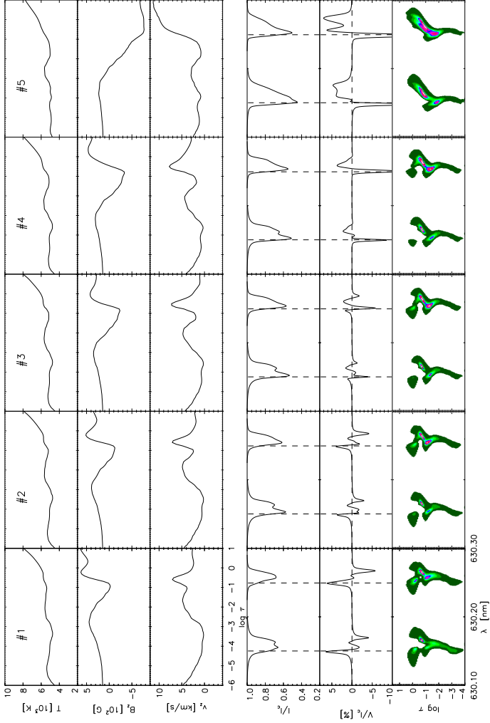
Figure 6.7: From top to bottom : Temperature, vertical component of magnetic field, vertical component of velocity, synthesized Stokes I and V profiles along the cut at t = 538 s shown in Fig. 6.5. Their position is marked by black vertical lines (from left to right).
