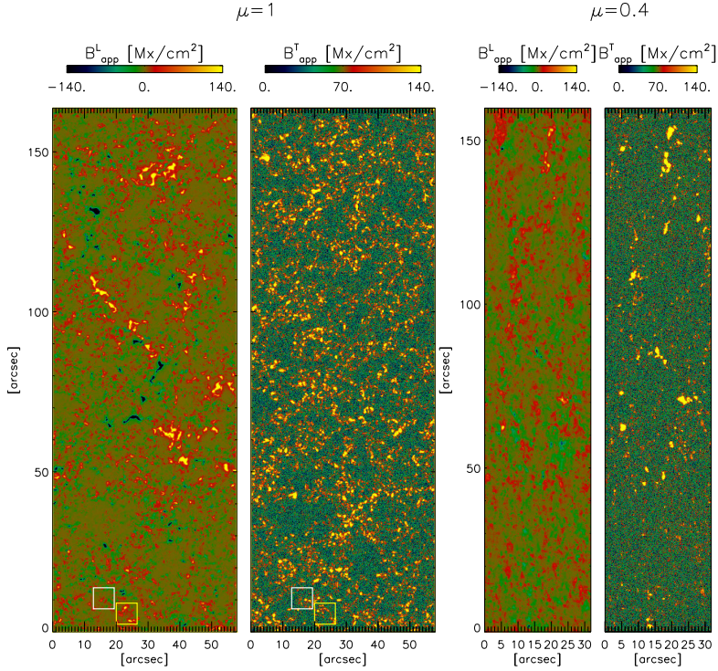
Figure 4.1: Maps of longitudinal ( B^L_{app} ) and transversal ( B^T_{app} ) apparent flux density for data set I (left) and III (right) from Table 4.2. The small squares indicate the sizes of the MHD snapshots. They also mark the position of the regions to which synthesized maps are compared (Figures 4.4 and 4.5)
