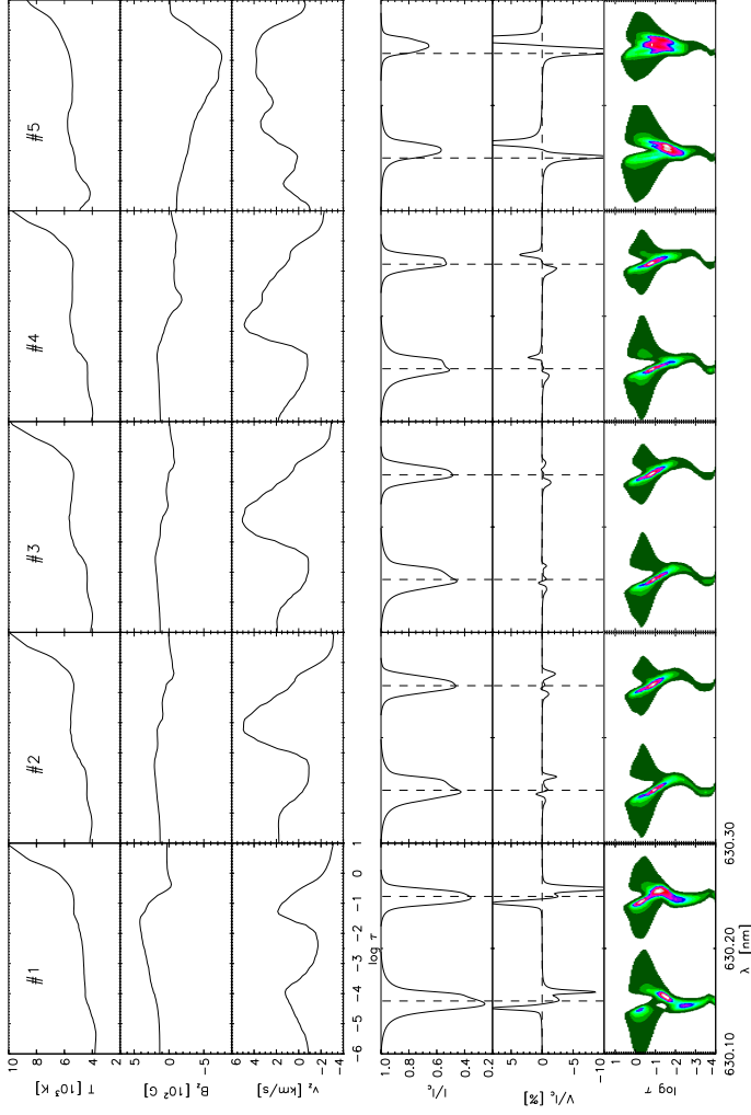
Figure 6.6: From top to bottom: Temperature, vertical component of magnetic field, vertical component of velocity, synthesized Stokes I and V profiles along the cut at t = 448 s shown in Fig. 6.5. Their position is marked by black vertical lines (from left to right).
