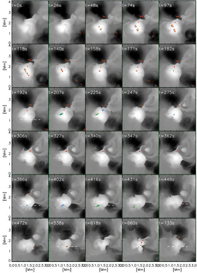
Figure 6.2: Time series of flux-cancellation events. The vertical magnetic field at \sim 600 km above \langle \tau_{500} \rangle = 1 is plotted. Red and blue contours mark dowflow of 5 km/s at \sim 80 km and upflow of 4 km/s at \sim 400 km above solar surface ( \langle \tau_{500} \rangle = 1 ), respectively. Green contours outline regions where upflow exceeds 9 km/s at \sim 600 km above the solar surface. White dashed lines show the position of the cuts plotted in Fig. 6.5. The grey scale is saturated at \pm 200 G.
