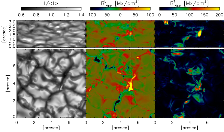
Figure 4.8: Apparent flux densities at the disc center (lower panels) and at \mu = 0.4 (upper panels) for a mixed-polarity (20 G) snapshot. From left to right: normalized continuum intensity, longitudinal and transversal apparent flux density.
