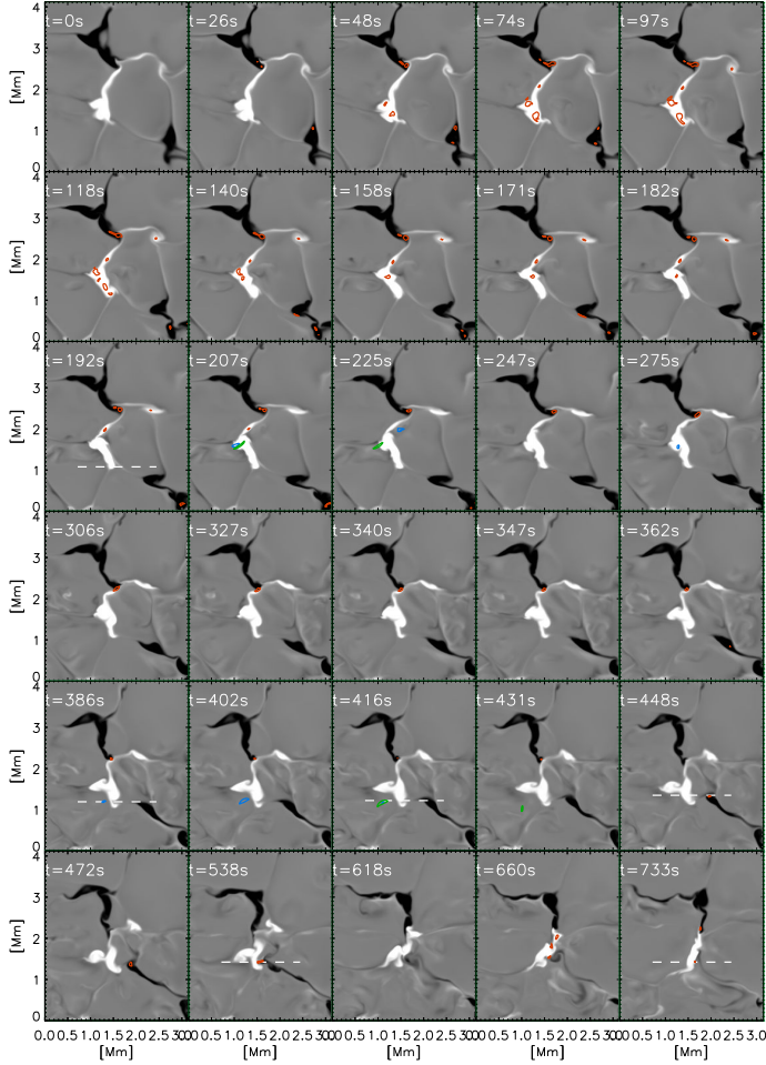
Figure 6.1: Time series of flux-cancellation events. The vertical magnetic field at \sim 80 km above \langle \tau_{500} \rangle = 1 is plotted. Red and blue contours mark dowflow of 5 km/s at \sim 80 km and upflow of 4 km/s at \sim 400 km above solar surface ( \langle \tau_{500} \rangle = 1 ), respectively. Green contours outline regions where upflow exceeds 9 km/s at \sim 600 km above the solar surface. White dashed lines show the position of the cuts plotted in Fig. 6.5. The grey scale is saturated at \pm 1000 G.
