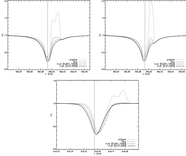
Figure 6.18: The change of the intensity profiles of the Fe II 5197.58 Å (lower panel) and Fe II 4923.92 Å (upper panels) when the effects of the terrestrial atmosphere are taken into account: SST telescope aperture ('Airy'), Lorentzian with a = 0.001 and b = 1000 km, and Lorentzian with a = 0.01 and b = 500 km. Representative profiles from the corresponding maps shown in Fig. 6.17.
