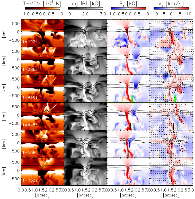
Figure 6.5: Vertical cuts through the regions marked by dashed lines in Figures 6.1, 6.2 and 6.3. From left to right: Temperature, magnetic field strength, vertical component of magnetic field and vertical component of velocity with overplotted velocity field in the x-z plane. The black horizontal lines mark the position of the \log \tau_{500} = 0, -1, -2 levels. The vertical lines mark the position of the pixels chosen to be studied in detail in Figures: 6.8 (orange), 6.9 (green), 6.6 and 6.7 (black).
