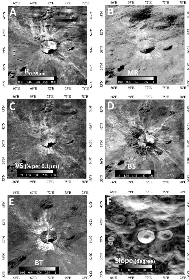
Fig. 6: Arruntia region from FC HAMO data ( \sim 60 m/pix). (A) Reflectance image at 0.55 \mu\text{m} . Derived band parameters: (B) MR (Mid Ratio), (C) VS (Visible Slope in % per 0.1 \mu\text{m} ), (D) BS ( 1\text{-}\mu\text{m} band strength), (E) BT (Band Tilt), (F) Surface (topographic) slope in degrees computed from HAMO-DTM ( \sim 62 m/pixel).
