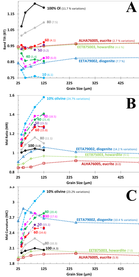
Fig. 3: Influence of grain size on (A) BT, (B) MR and (C) MC parameters, for HEDs in size ranges <25, 25-45, 45-75, 75-125, 125-250, 250-500 \mu\text{m} , and olivine-orthopyroxene mixtures (10-90% Olivine) and 100% olivine in size ranges <38, 38-53, 63-90, 90-125 \mu\text{m} . The maximum variations (%) of each sample over the whole grain size ranges are given in brackets. Data points for some of the mixtures are not shown to enhance readability.
