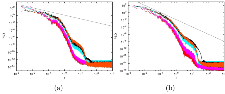
FIG. 3.10: Numerical results of the reversing gravitational dynamo at Ra = 1 \cdot 10^6 , Pm = 5.75, 6, 13, 20, 25, 35 , E = 6.5 \cdot 10^{-5} and Pr = 1 . a) PSD of u_{rms} . b) PSD of B_{rms} .
