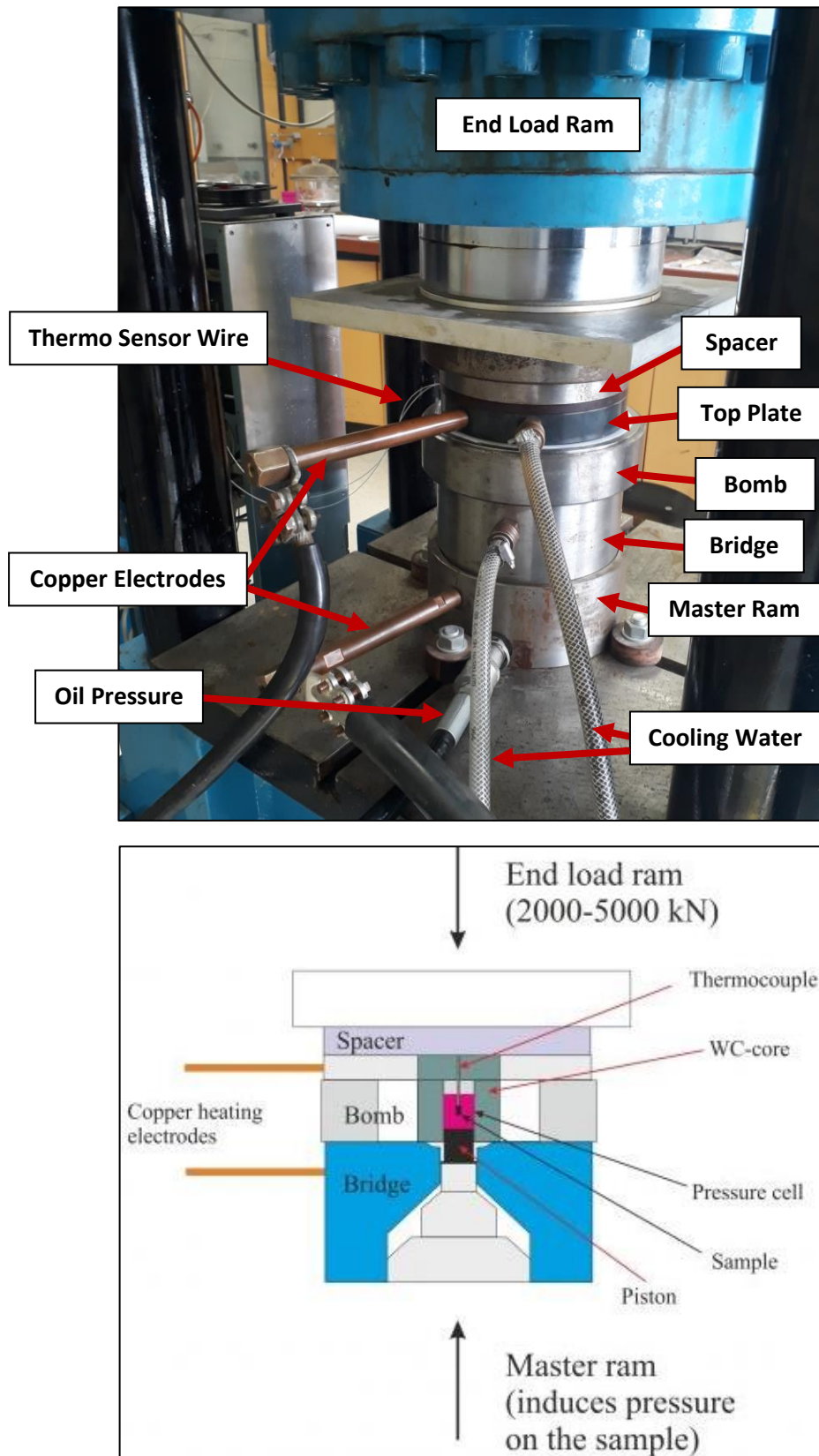
Figure 15: End-load piston cylinder press of the GZG (top) and schematic structure (bottom). The end-load gives the materials the necessary strength to withstand the pressure generated, while the master ram from below generates the actual pressure on the sample. (Scheme by Dr Enikő Bali, http://enikobali.huPont.hu )
