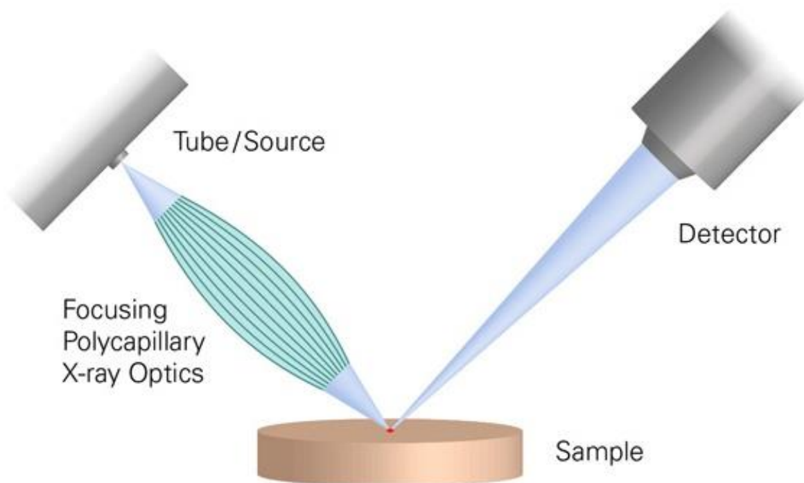
Figure 58: Schematic representation of the X-ray optics of a Bruker M4 "Tornado".
