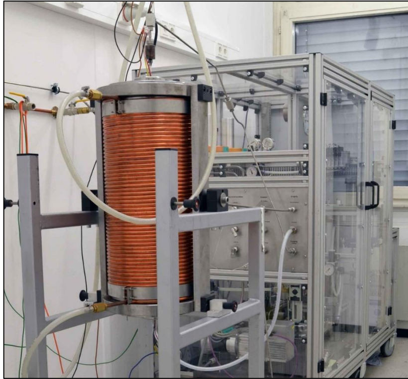
Figure 21: Internally Heated Pressure Vessel (IHPV) of the GZG. In front is the autoclave with cooling water connections, behind it is the plexiglass cabinet with the pressure amplifiers and pressure lines.
