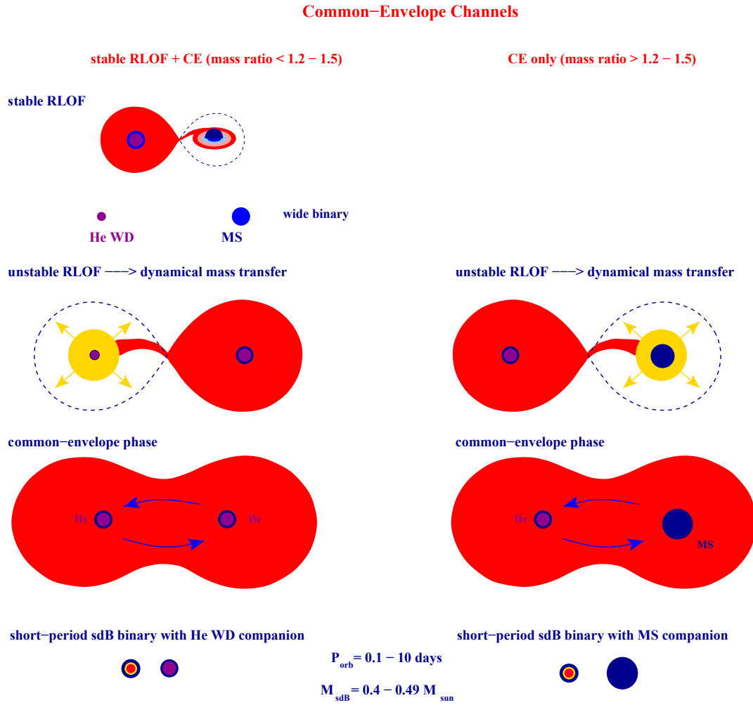
Figure 2.4: Common-envelope (CE) channels for the production of sdB stars. The CE phase can be either the first (right panel) or the second (left panel) mass-transfer phase, producing a tight sdB binary with either a normal-star or white-dwarf companion, respectively (Podsiadlowski 2008). By the kind permission of ASP Conference Series, vol. 401, P. Podsiadlowski, p. 63.
