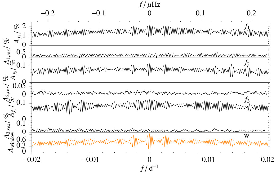
Figure 9.5: Amplitude spectrum of QQ Vir of the main pulsation frequency f_1 = 626.877628 \text{ d}^{-1} (top), f_2 = 552.00713 \text{ d}^{-1} (top middle), f_3 = 642.0516 \text{ d}^{-1} (bottom middle) with the respective residuals after the pre-whitening below and the normalised window-function (bottom).
