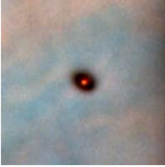
Figure 2.2: Left: Protoplanetary disc imaged by the Hubble Space Telescope in the Orion nebula. The image is about 1800 au across. Credit: NASA, C.R. O’Dell and S.K. Wong. Right: ALMA image of HL Tauri showing the protoplanetary disc at a wavelength of 1.3 mm. The image is about 250 au across. Credit: ALMA (ESO/NAOJ/NRAO).
